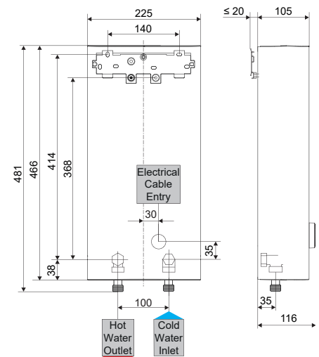
Dimensions and Connections
